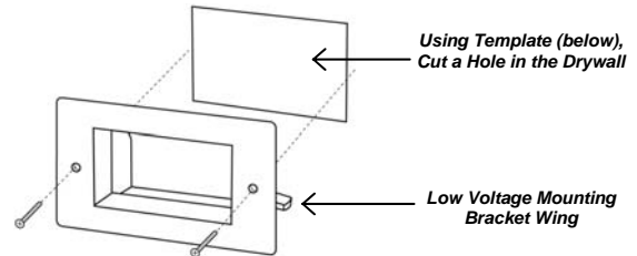
Figure 2 - Front View
