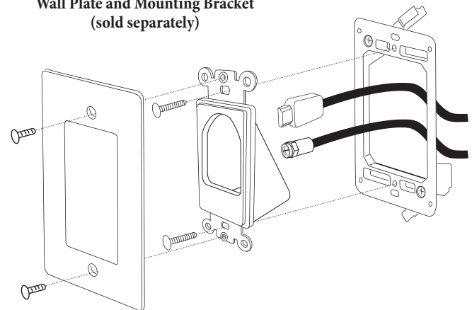
Installation Diagram
