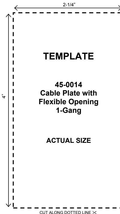
Figure 2 - Front View
