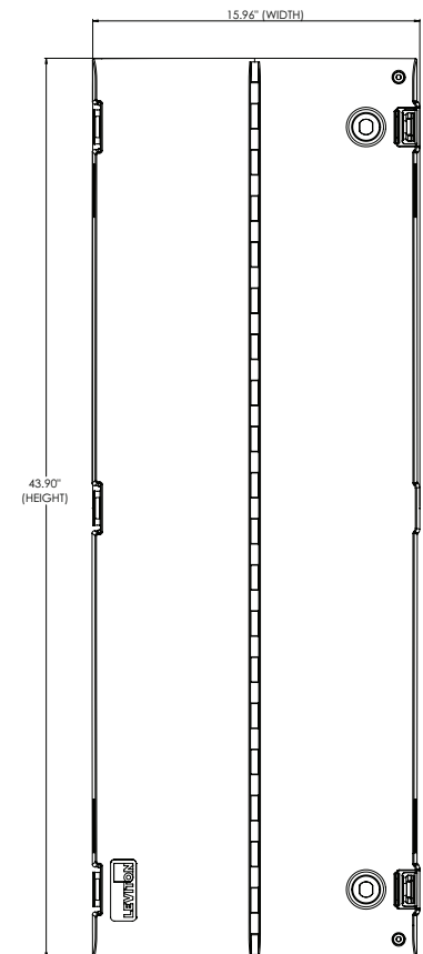
42-Inch Vented Hinged Door
