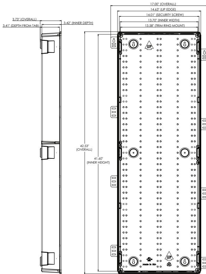
42-Inch Structured Media Center Enclosure
