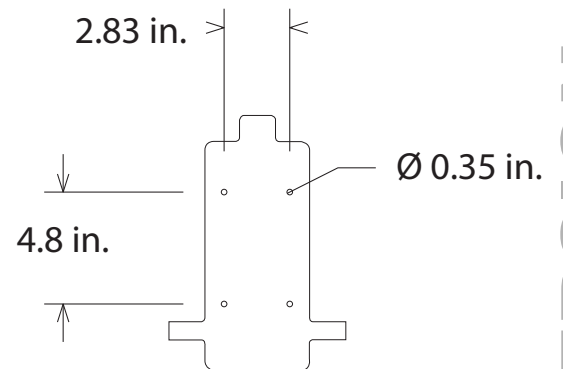
Mounting Bracket
