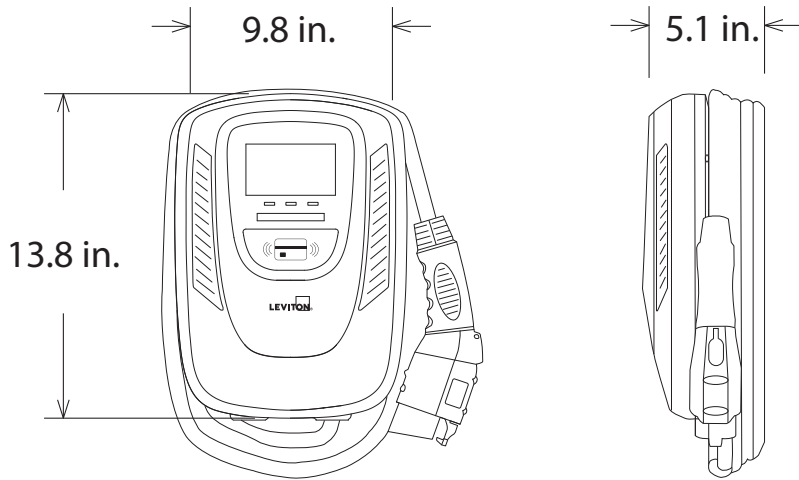
Main Size of Charger - EV48S
