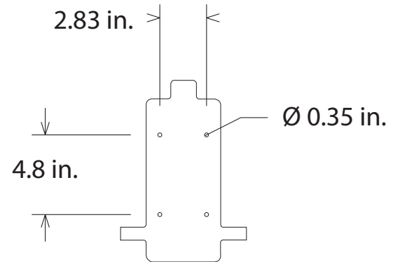
Mounting Bracket
