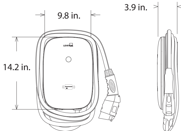
Main Size of Charger - EV320, EV32W and EV48W
