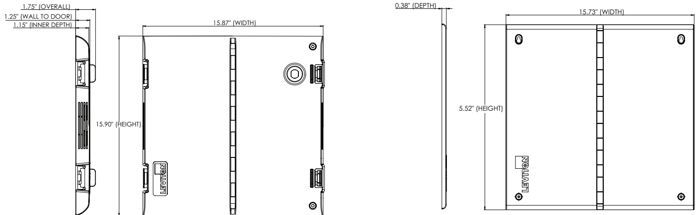
14-Inch Vented Cover
