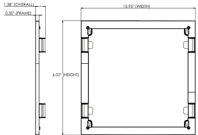
14-Inch Trim Ring Accessory
